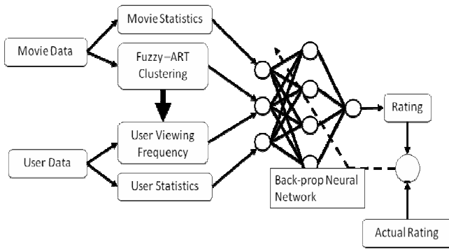
Figure 6 – Overview of Modeling Architecture
