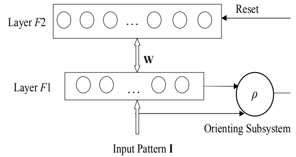
Figure 7 - Topological structure of Fuzzy ART. Layers F_1 and F_2 are connected via adaptive weights W . The orienting subsystem is controlled by the vigilance parameter \rho .
