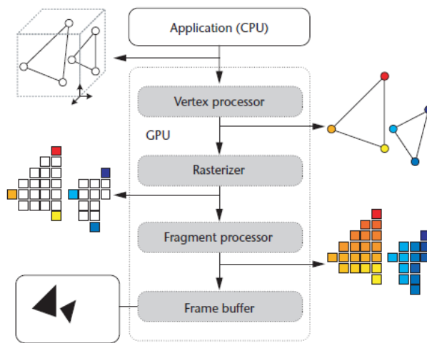
Fig 2. The graphics processing pipeline. Modern GPU's combine the vertex and fragment processor into a unified shader unit that is able to perform either of these functions. Currently, GPU's can include up to 128 unified shader units. Figure Courtesy of Goodnight [2].
