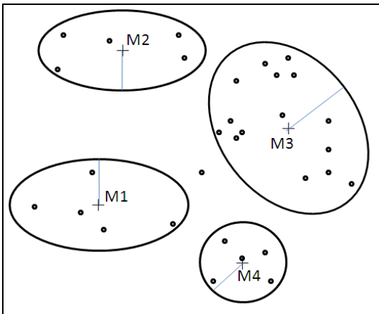
Figure 13. TSP Instance after first clustering pass. Each cluster initializes a meme, labeled with "M#" and a "+" denoting the centroid.
