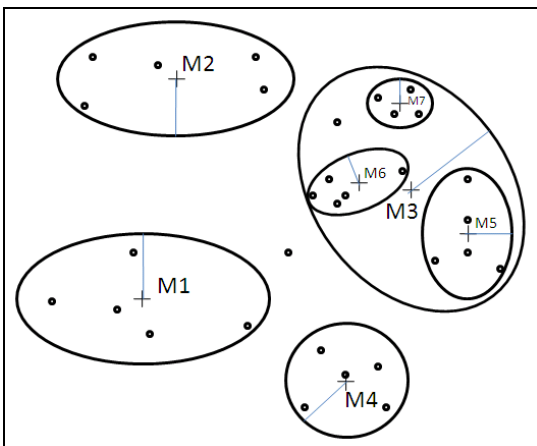
Figure 14. Second clustering pass. Note the new clusters, M5, M6, and M7.
