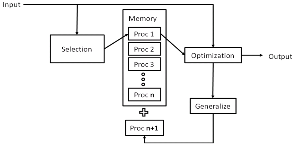
Figure 2. Meta-Learning Architecture
