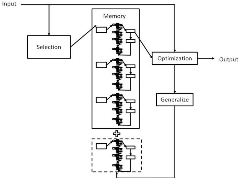
Figure 4. N^{\text{th}} -order Meta Learning
