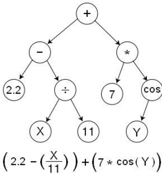
Figure 5. Illustration of function representation as tree structure.
