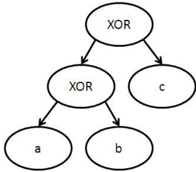
Figure 9. Simplified three-input XOR.
