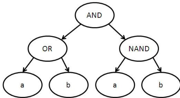
Figure 6. XOR tree representation.
