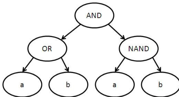
Figure 10. Initial non-meta learning XOR2 individual.
