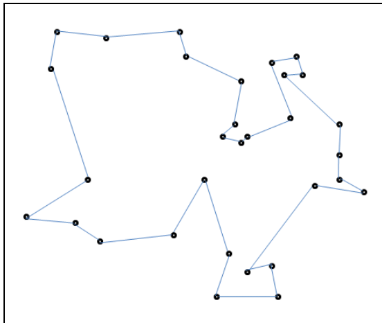
Figure 20. Completed tour.
