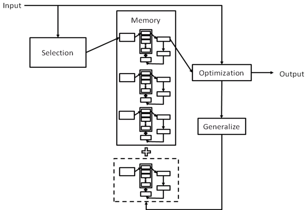
Figure 3. Meta-Meta Learning
