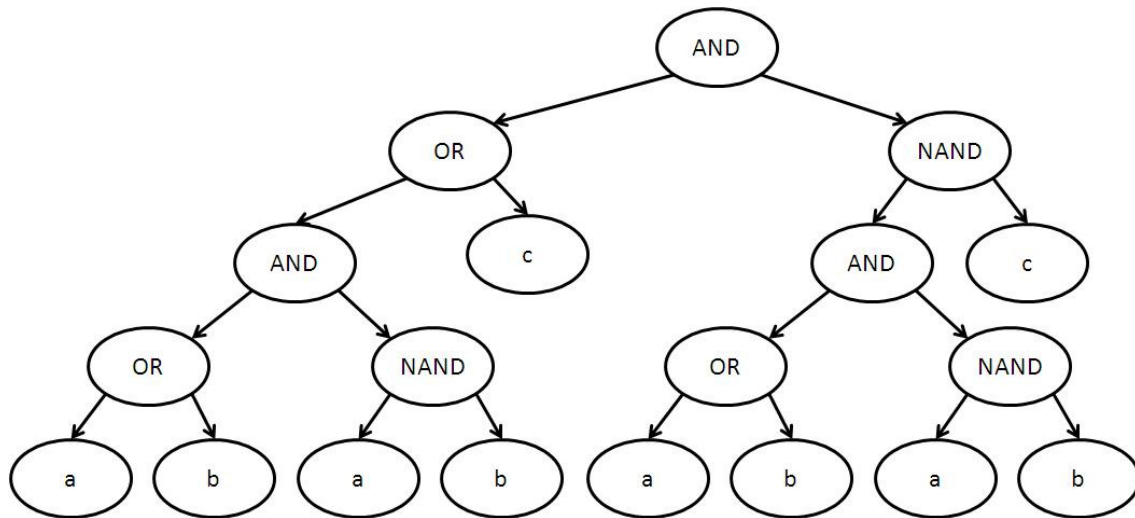
Figure 7. Three-input XOR tree representation.
