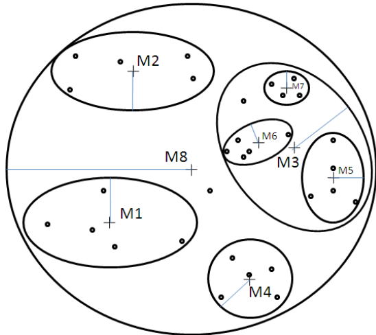
Figure 15. Final clustering pass, with global cluster M8
