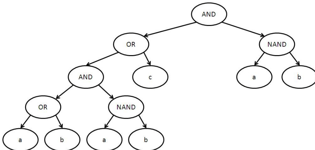
Figure 11. Intermediate step in development of 3-bit XOR function after a single generation.
