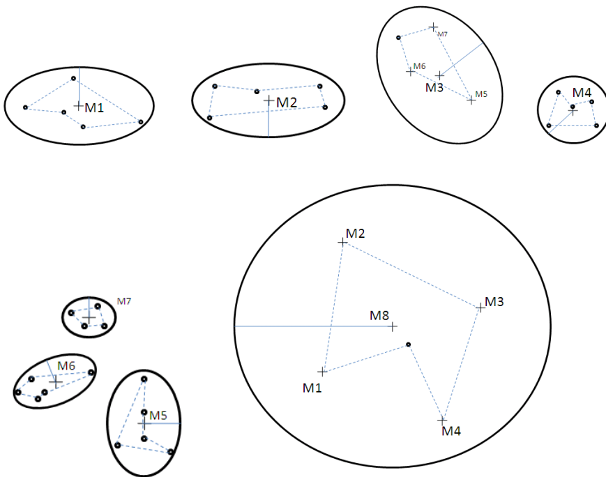
Figure 17. Completed memes, M1 through M8. Super-clusters reference the centroids of sub-clusters. Note that memes M2 and M4 are similar in structure, but not scale.
